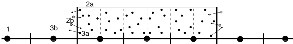
Figure 1: Schematic representation of the coupling mechanisms of the hybrid algorithm. 1. Advance continuum solution. 2. Advance DSMC solution (2a), using continuum data in reservoir boundaries (2b). 3. Reflux (3a) to correct continuum solution near interface (3b).
