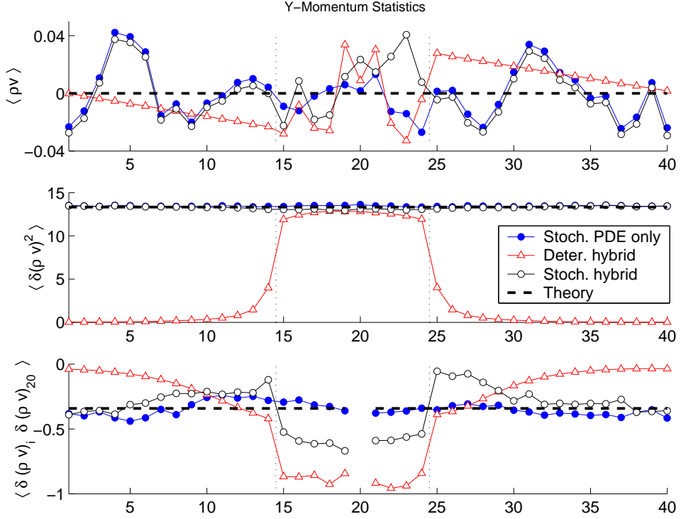
Figure 4: Mean, variance, and center point correlation of y -momentum versus spatial location for a system at equilibrium. Vertical dotted lines depict the boundaries of the particle region, for both hybrids. Note that, for clarity, the correlation value at i = j = 20 is omitted from the plot.
